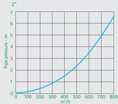
□ Discharge capacity (free air flow)
