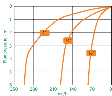
□ Inflow data (free air flow) ½", ¾" & 1"
