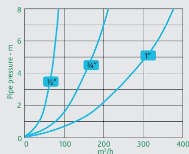
□ Discharge capacity (free air flow) ½", ¾" & 1"
