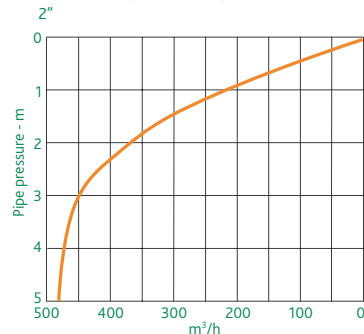
□ Inflow data (free air flow)
